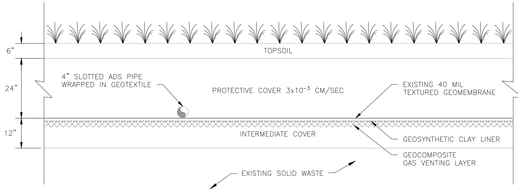
EXISTING FINAL COVER SLOPES LESS THAN 25 PERCENT
