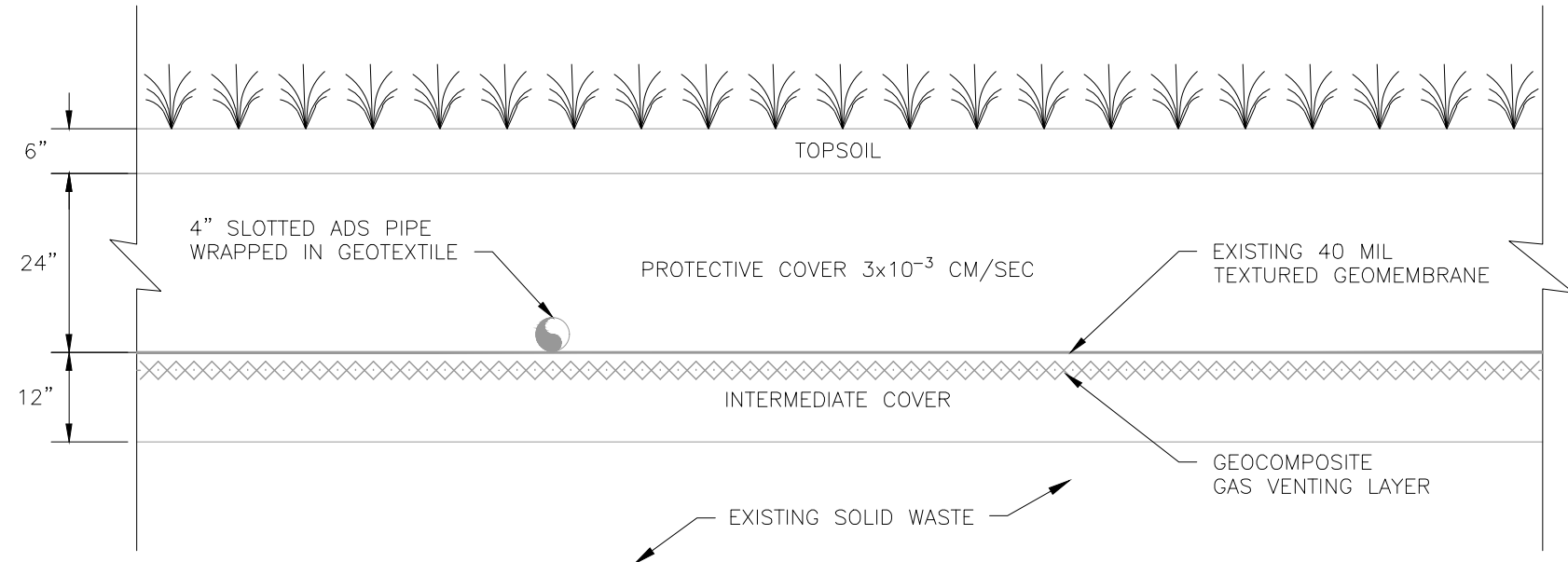
EXISTING FINAL COVER SLOPES GREATER THAN 25 PERCENT
