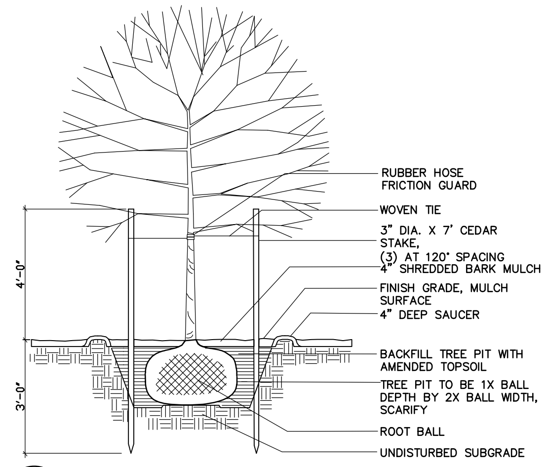
1 TYPICAL TREE PLANTING
